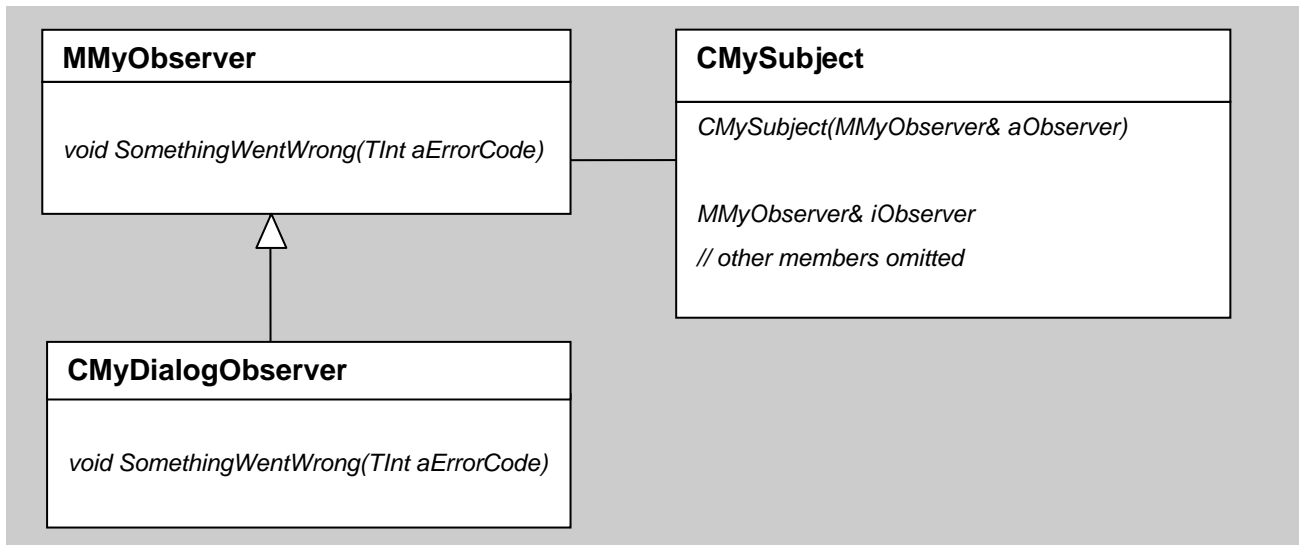
Figure 1: the 'Observer' pattern
