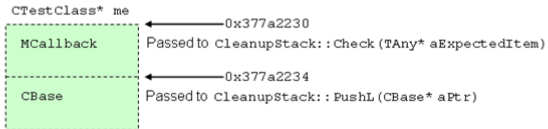
Figure 1 : The layout of CTestClass (taken from [2])
